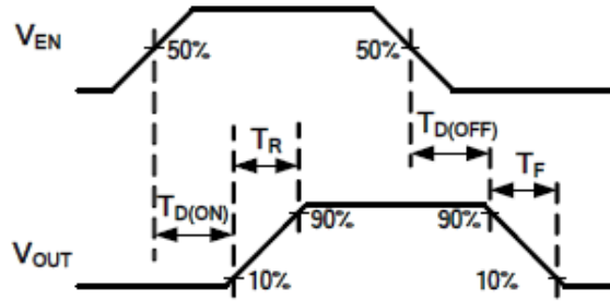
Figure 1. Voltage Waveforms: AP2155
