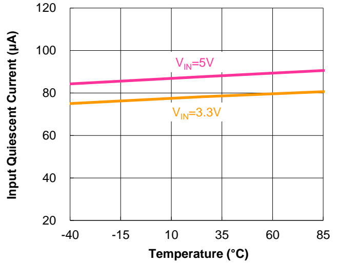
Input Quiescent Current vs. Temperature
