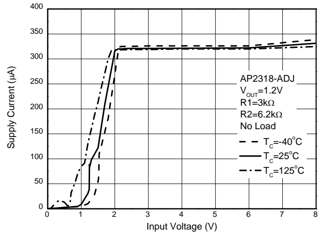
Supply Current vs. Input Voltage (Conditions: V_{OUT} = 1.2V , R1 = 3k\Omega , R2 = 6.2k\Omega )
