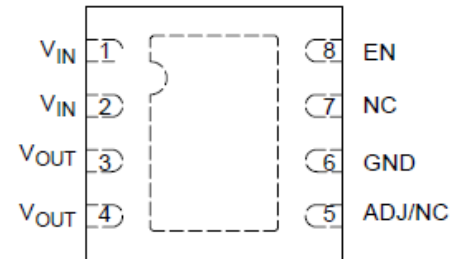
DFN-3x3-8
