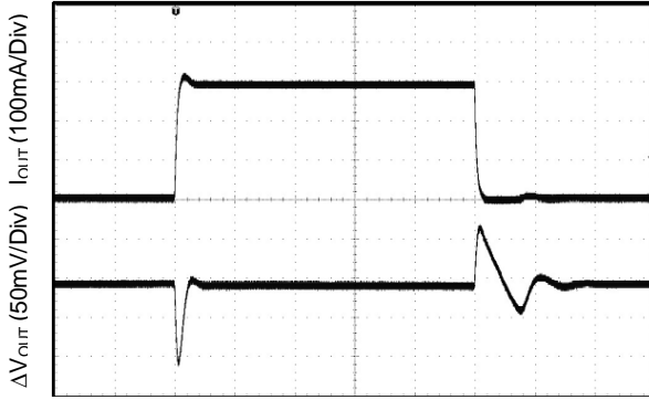
Time (200μs/Div)
