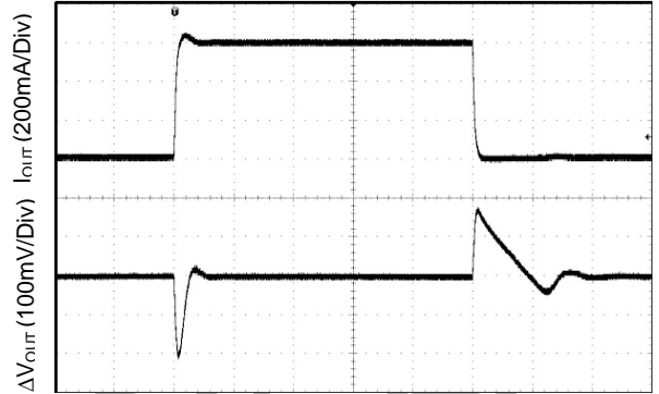
Time (200μs/Div)
