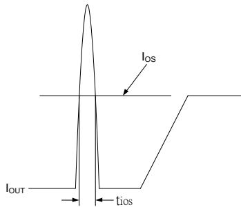
Figure 1. Output Short-Circuit Timing Diagram
