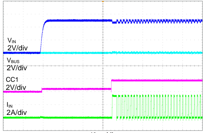
IN1 = IN2 = AUX = EN = CHG = CHG\_HI = 5\text{V} , CC1 = Rd , CC2 = \text{open} , OUT = \text{shorted} Figure 14. Hot-Plug to Short
