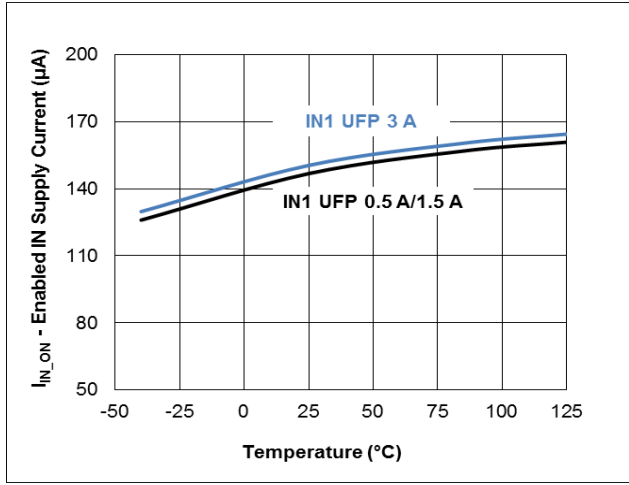
Figure 8. IN1 Current with UFP vs. Temperature
