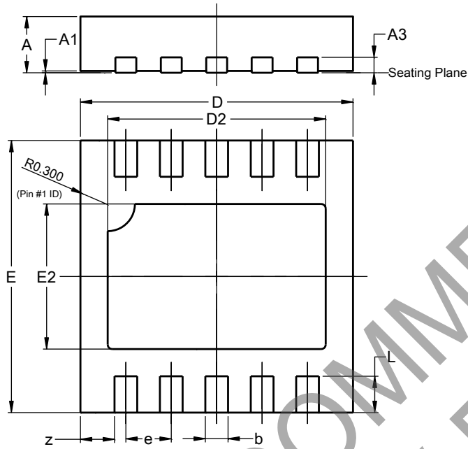
U-DFN3030-10
