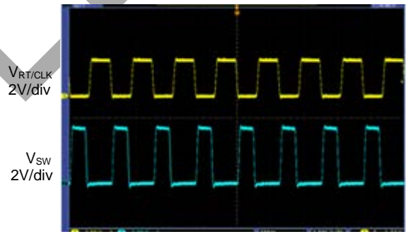
Time 400ns/div Figure 4. Synchronizing Waveform
