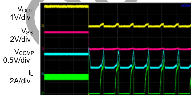
Time 3.2ms/div
