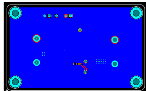
Figure 7. Bottom View of PCB Layout
