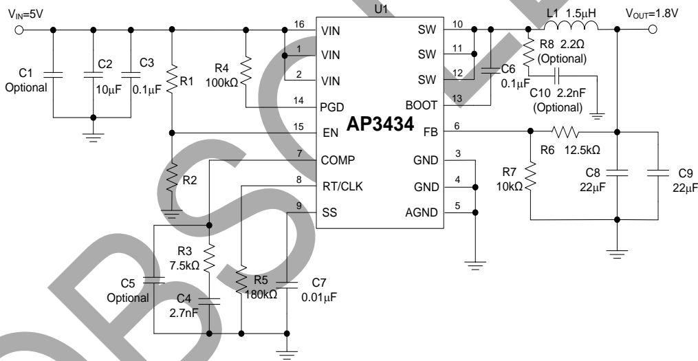
Figure 5. Typical Application of AP3434
