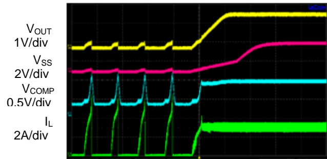
Time 3.2ms/div
