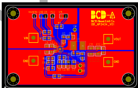
Figure 6. Top View of PCB Layout
