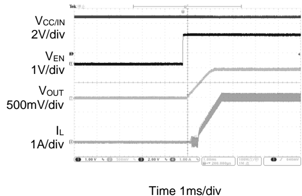
Enable Waveform ( V_{IN}=V_{CC}=5V , V_{OUT}=1V , I_{OUT}=3A )
