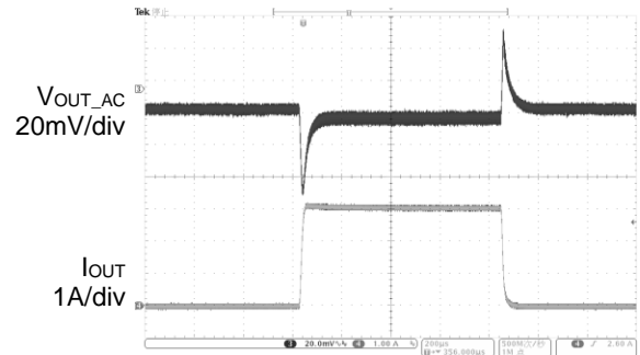
Load Transient Response ( V_{IN}=V_{CC}=5V , V_{OUT}=1V , I_{OUT}=0 to 3A)
