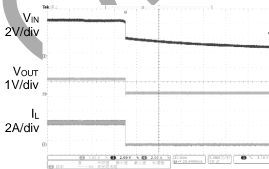
Power off Waveform ( V_{IN}=V_{CC}=5V , V_{OUT}=1V , I_{OUT}=3A )
