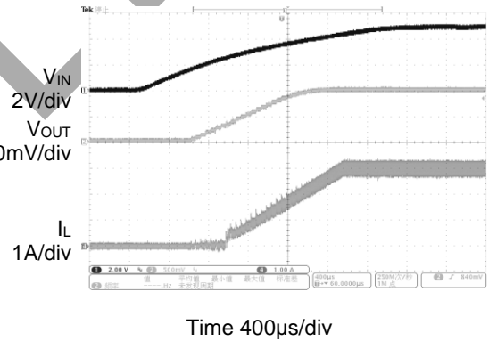
Power on Waveform ( V_{IN}=V_{CC}=5V , V_{OUT}=1V , I_{OUT}=3A )
