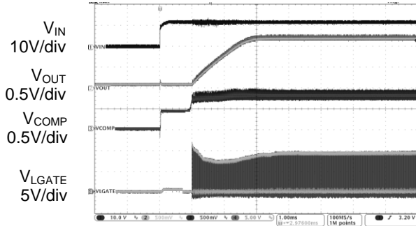
Power-on Waveform ( V_{IN}=12V , V_{OUT}=1.2V , I_{OUT}=0A )
