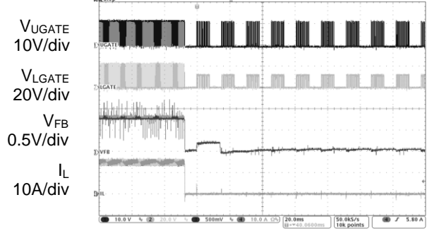
Under Voltage Protection ( V_{IN}=12V , V_{OUT}=1.2V , I_{OUT}=20A )
