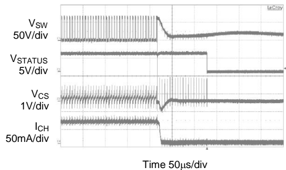
Schottky/Inductor Short Protection
