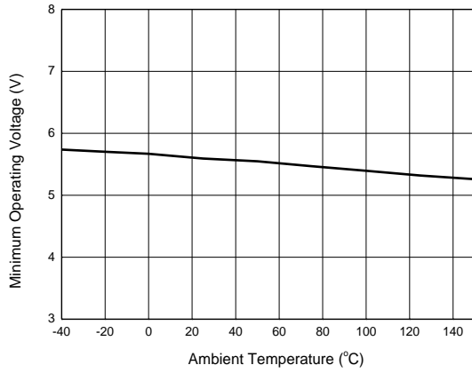
Figure 12. Minimum Operating Voltage vs. Ambient Temperature
