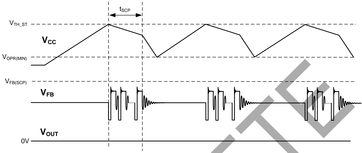
Figure 9. Short Circuit Protection (SCP) and Hiccup Mode
