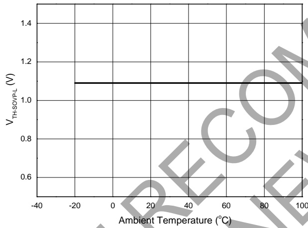
V TH-SOVP-L vs. Ambient Temperature
