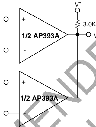
ORing the Outputs
