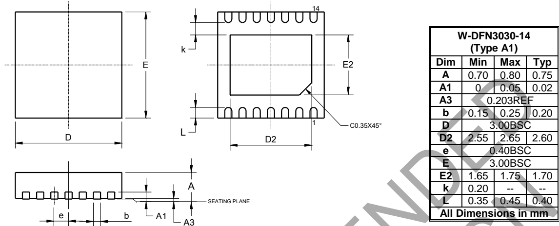
W-DFN3030-14 (Type A1)
