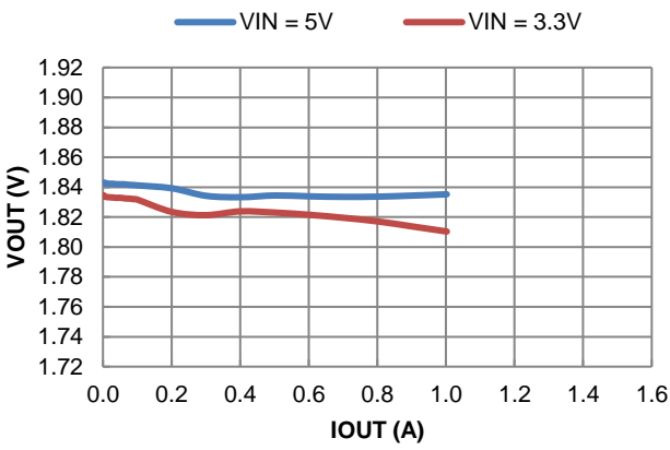
Figure 24. Load Regulation
