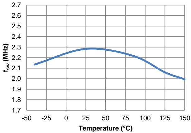
Figure 26. f_{sw} vs. Temperature, I_{OUT} = 0\text{A}
