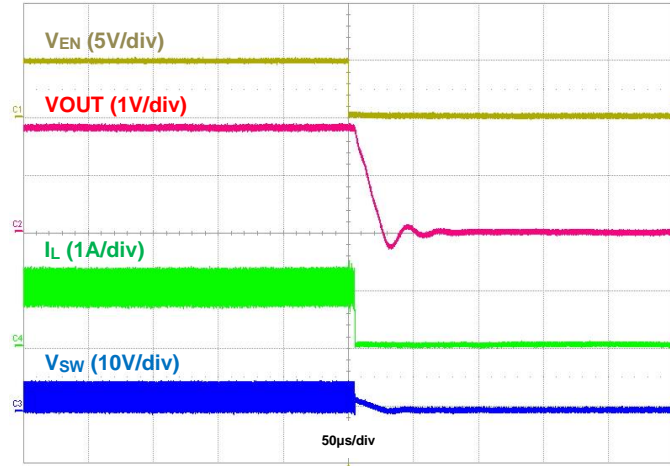
Figure 34. Shutdown Using EN, IOU = 1A
