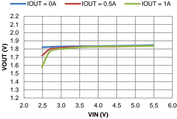
Figure 23. Line Regulation
