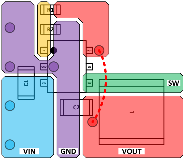
Figure 42. Recommended AP61100Q PCB Layout
