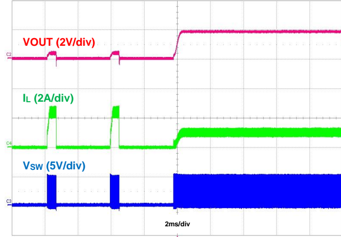
Figure 36. Output Short Recovery, IOU = 1A
