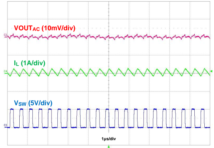
Figure 28. Output Voltage Ripple, I_{OUT} = 50\text{mA}
