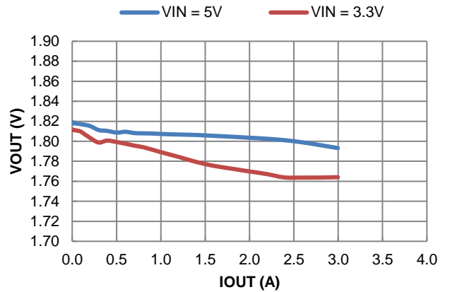
Figure 24. Load Regulation
