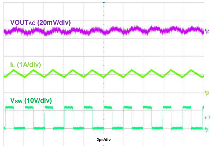
Figure 15. Output Voltage Ripple, V_{OUT} = 5\text{V} , I_{OUT} = 1\text{A}
