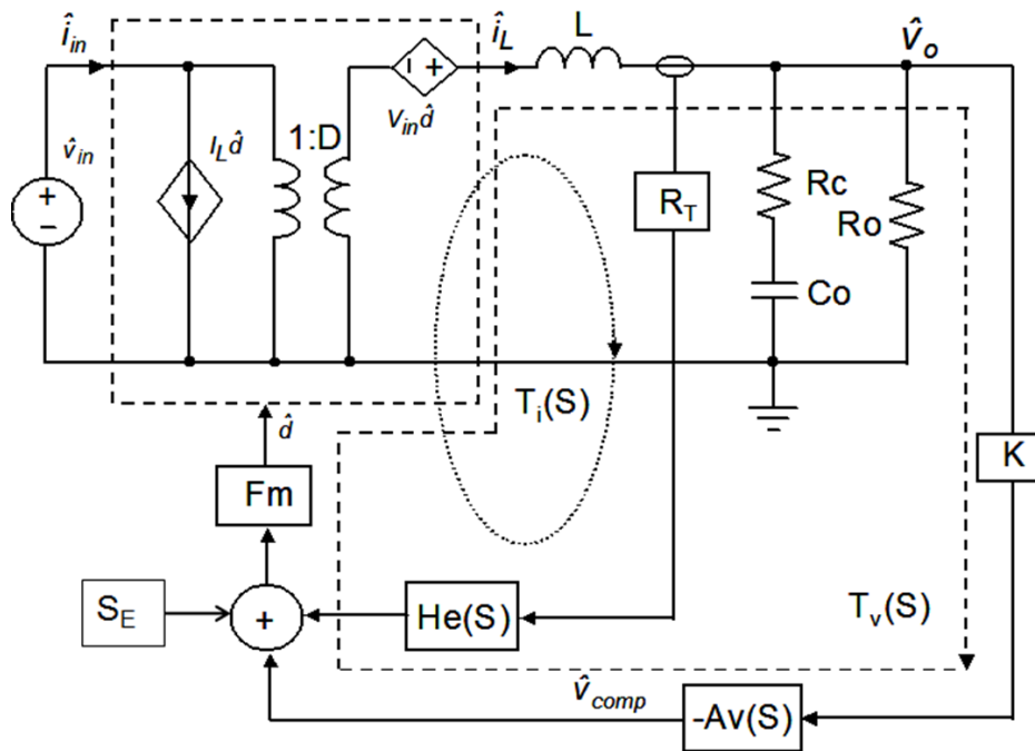
Figure 45. Linearized Small-Signal Model
