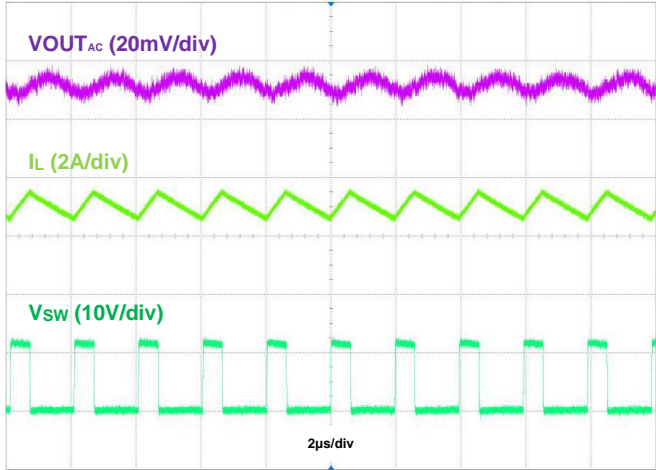
Figure 23. Output Ripple, V_{IN} = 12\text{V} , V_{OUT} = 3.3\text{V} @3A, PFM
