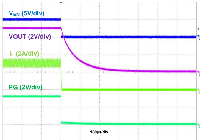
Figure 34. Shutdown using EN with PG, IOUT = 3A
