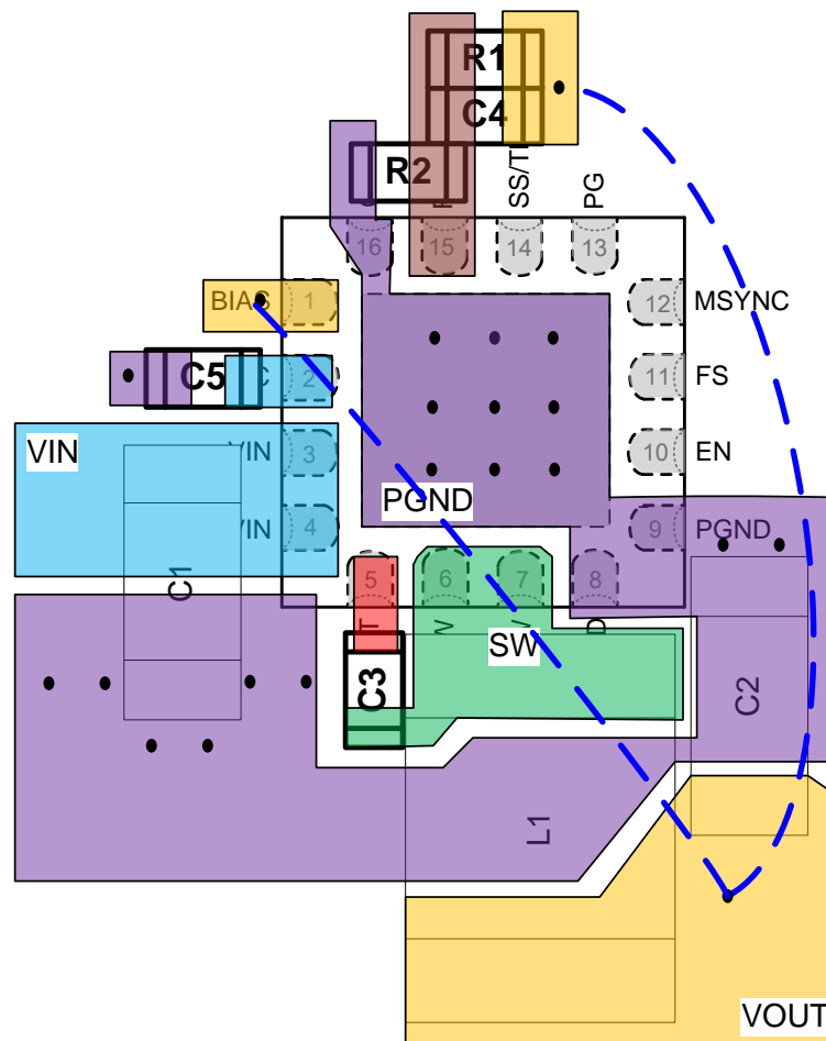
Figure 47. PC Board Layout
