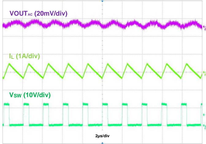
Figure 24. Output Ripple, V_{IN} = 12\text{V} , V_{OUT} = 3.3\text{V} @50mA, PFM
