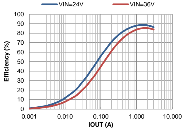
Figure 8. PWM Efficiency vs. Output Current, V_{OUT} = 3.3\text{V} , L = 5.5\mu\text{H}
