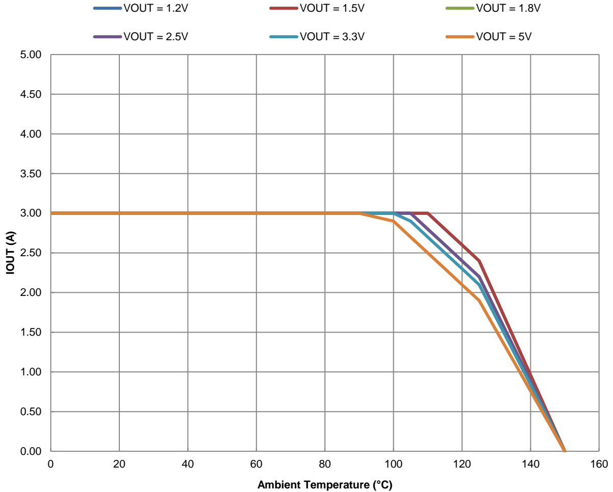
Figure 41. Output Current Derating Curve vs. Ambient Temperature, VIN = 12V
