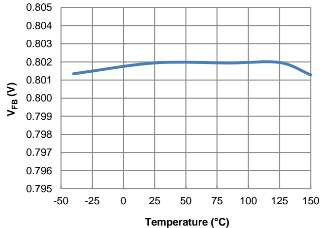
Figure 10. Feedback Voltage vs. Temperature
