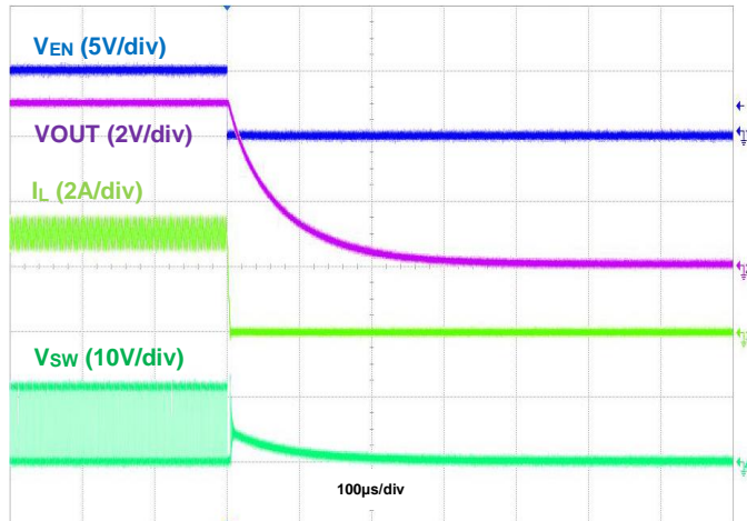
Figure 32. Shutdown using EN, IOUT = 3A
