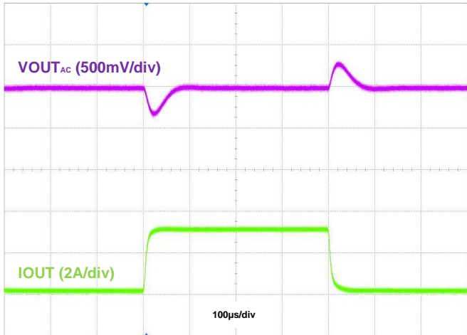
Figure 29. Load Transient, IOUT = 50mA to 3A to 50mA, PWM
