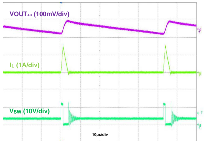
Figure 22. Output Ripple, V_{IN} = 12\text{V} , V_{OUT} = 3.3\text{V} @50mA, PFM
