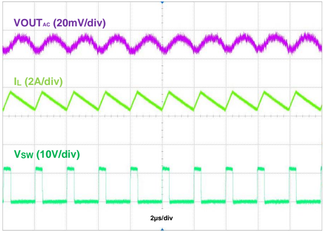
Figure 17. Output Ripple, V_{IN} = 12\text{V} , V_{OUT} = 5\text{V} @3A, PFM
