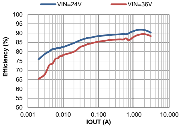
Figure 5. PFM Efficiency vs. Output Current, V_{OUT} = 5\text{V} , L = 6.5\mu\text{H}
