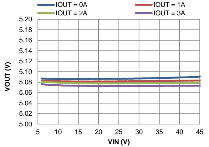
Figure 14. Line Regulation
