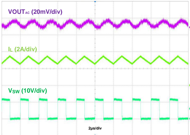
Figure 19. Output Ripple, V_{IN} = 12\text{V} , V_{OUT} = 5\text{V} @3A, PWM
