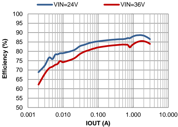
Figure 7. PFM Efficiency vs. Output Current, V_{OUT} = 3.3\text{V} , L = 5.5\mu\text{H}
