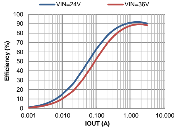
Figure 6. PWM Efficiency vs. Output Current, V_{OUT} = 5\text{V} , L = 6.5\mu\text{H}
