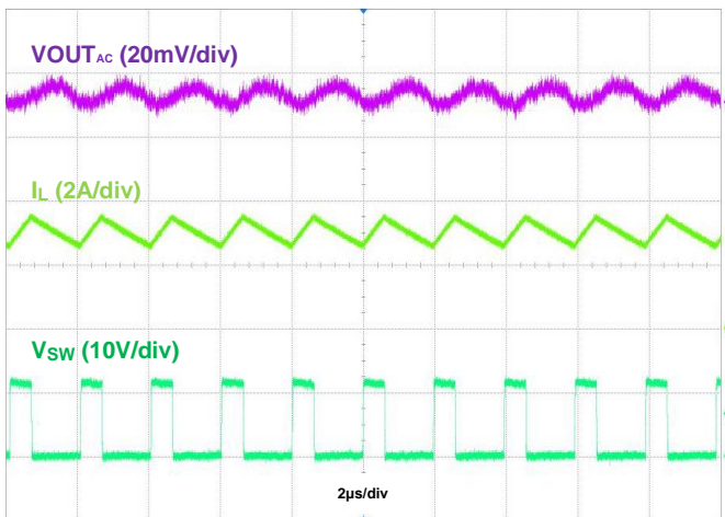
Figure 21. Output Ripple, V_{IN} = 12\text{V} , V_{OUT} = 3.3\text{V} @3A, PFM
