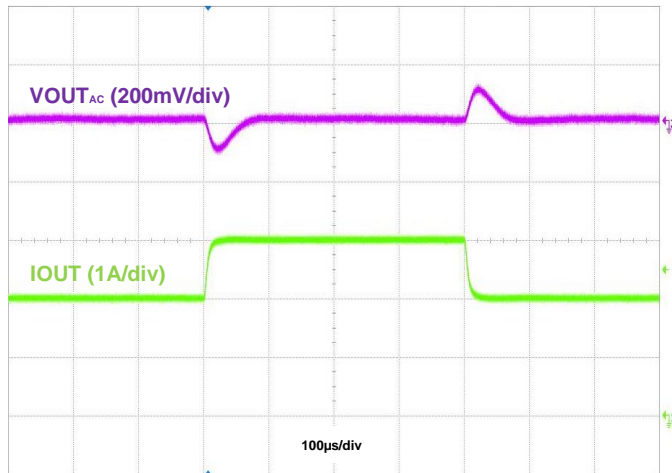
Figure 28. Load Transient, I_{OUT} = 2\text{A} to 3A to 2A, PFM
