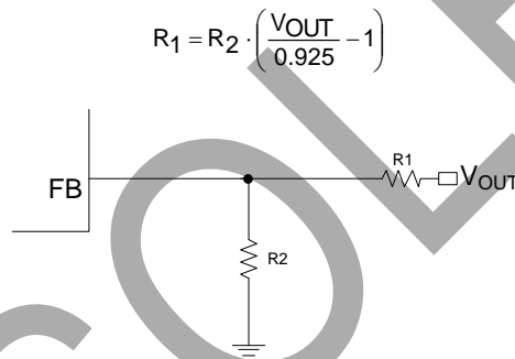
Figure 3 Feedback Divider Network
