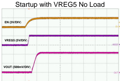
Time-1ms/div
