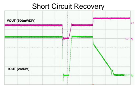
Time-500μs/div
