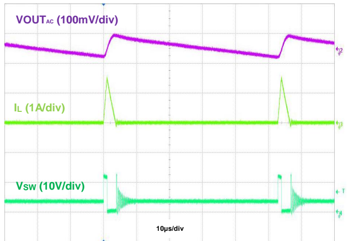
Figure 22. Output Ripple, V_{IN}=12\text{V} , V_{OUT} = 3.3\text{V} @50mA, PFM
