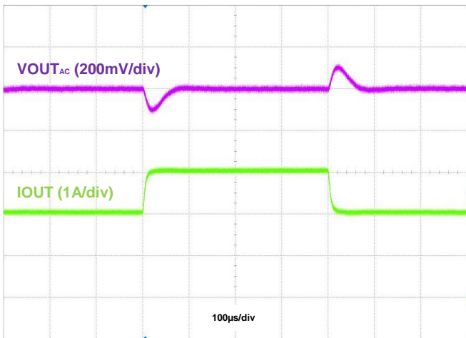
Figure 27. Load Transient, I_{OUT} = 2\text{A} to 3A to 2A, PWM
