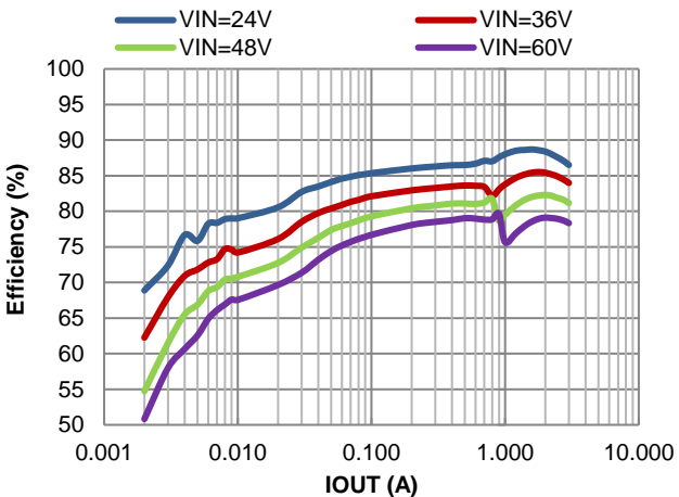
Figure 7. PFM Efficiency vs. Output Current, V_{OUT}=3.3\text{V} , L=5.5\mu\text{H}
