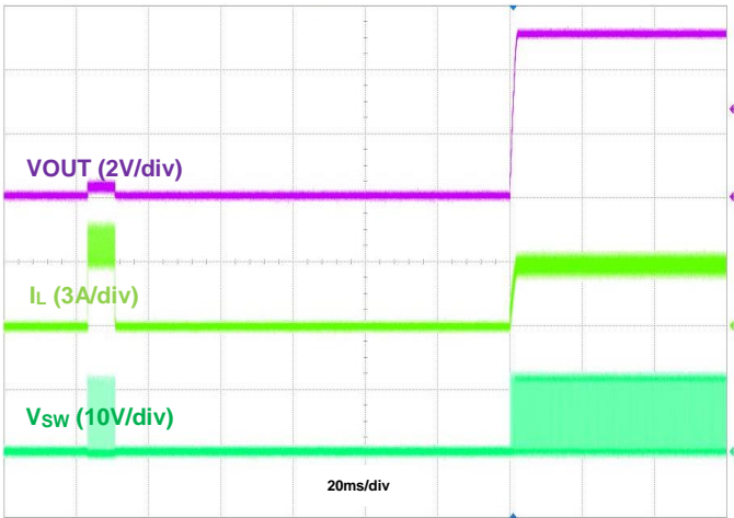
Figure 36. Output Short Recovery, I_{OUT} = 3\text{A}
