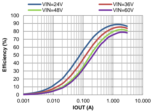
Figure 8. PWM Efficiency vs. Output Current, V_{OUT}=3.3\text{V} , L=5.5\mu\text{H}
