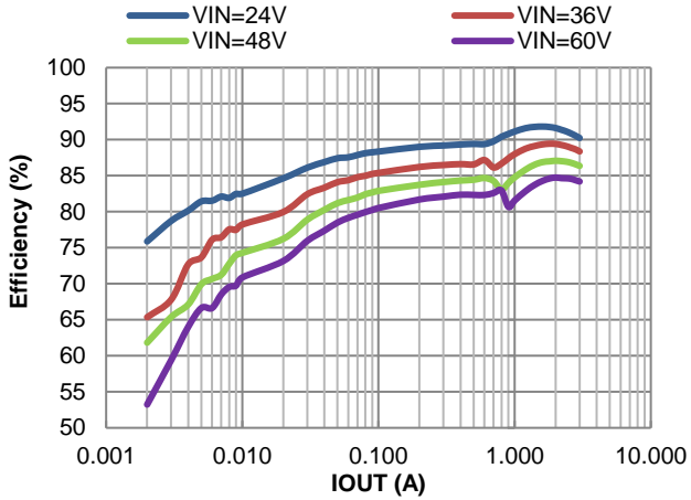
Figure 5. PFM Efficiency vs. Output Current, V_{OUT}=5\text{V} , L=6.5\mu\text{H}
