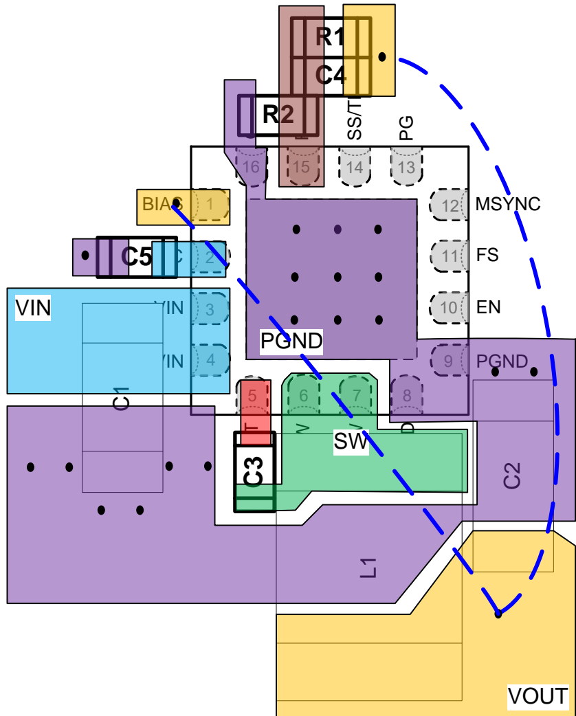
Figure 47. PC Board Layout
