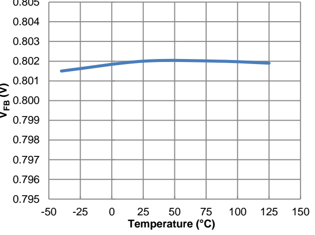
Figure 10. Feedback Voltage vs. Temperature
