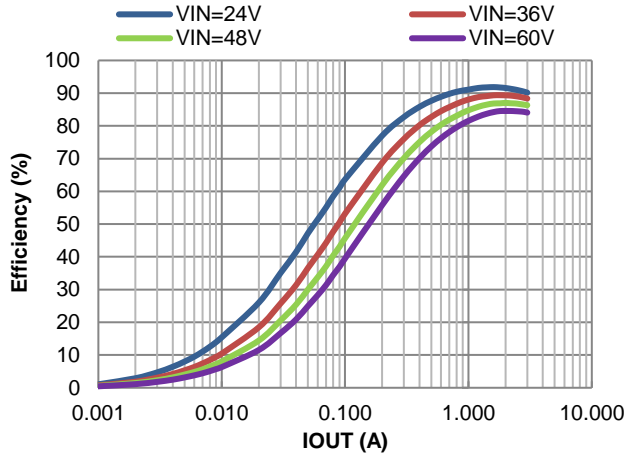
Figure 6. PWM Efficiency vs. Output Current, V_{OUT}=5\text{V} , L=6.5\mu\text{H}
