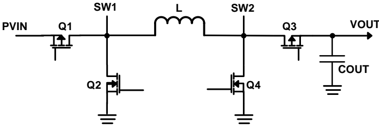
Figure 2. Buck-Boost Diagram
