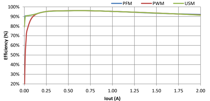
Efficiency, P VIN =3.3V, V OUT =3.4V
