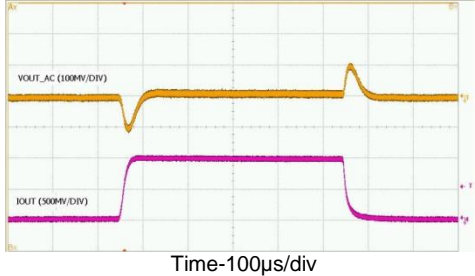
Load Transient (V IN =5.5V, PWM, I O =0 to 1A)
