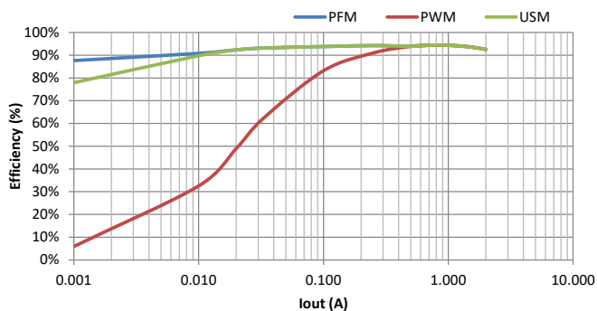
Efficiency, P VIN =5V, V OUT =3.4V
