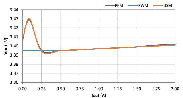
Load Regulation, P VIN =3.3V, V OUT =3.4V
