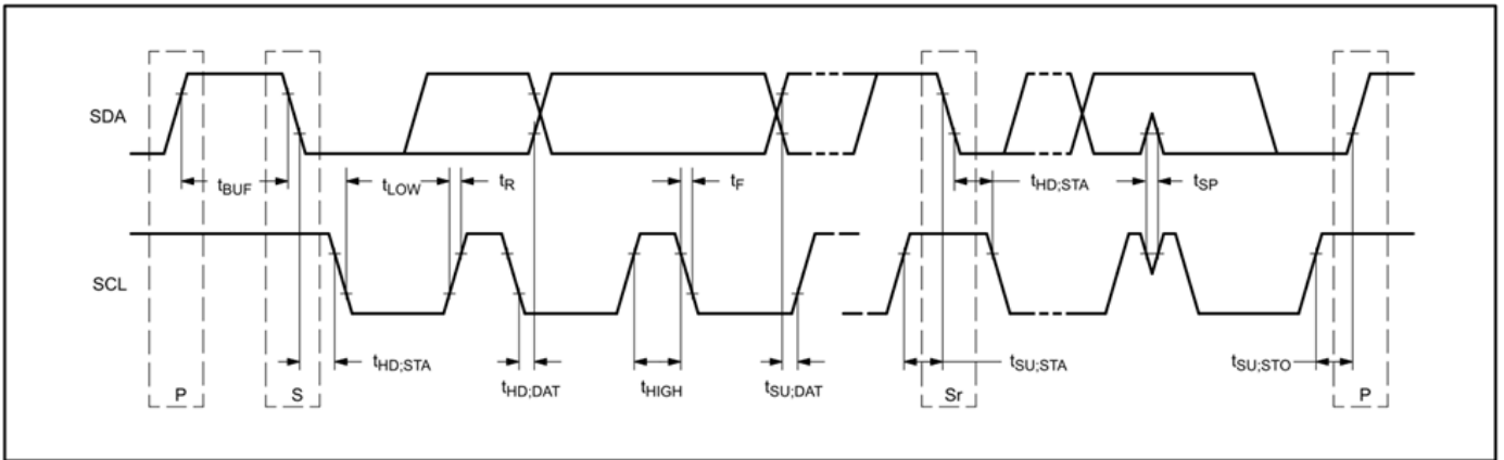
Figure 5. Start and Stop Conditions
