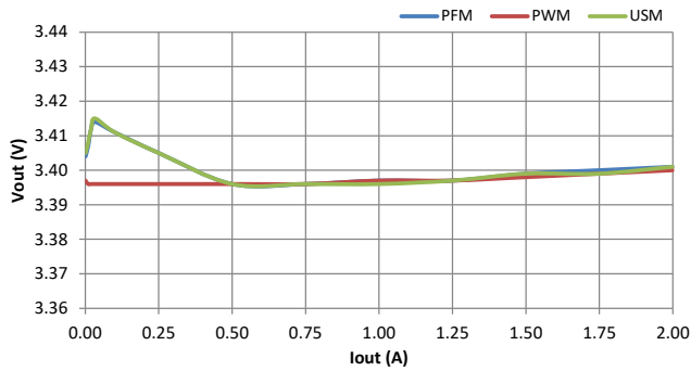
Load Regulation, P VIN =5V, V OUT =3.4V
