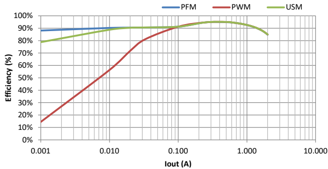
Efficiency, P VIN =2.7V, V OUT =3.4V
