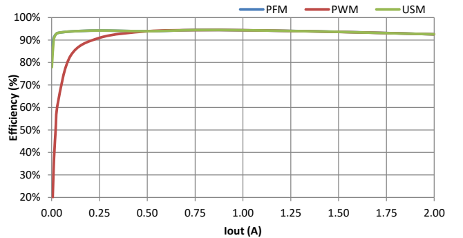
Efficiency, P VIN =5V, V OUT =3.4V
