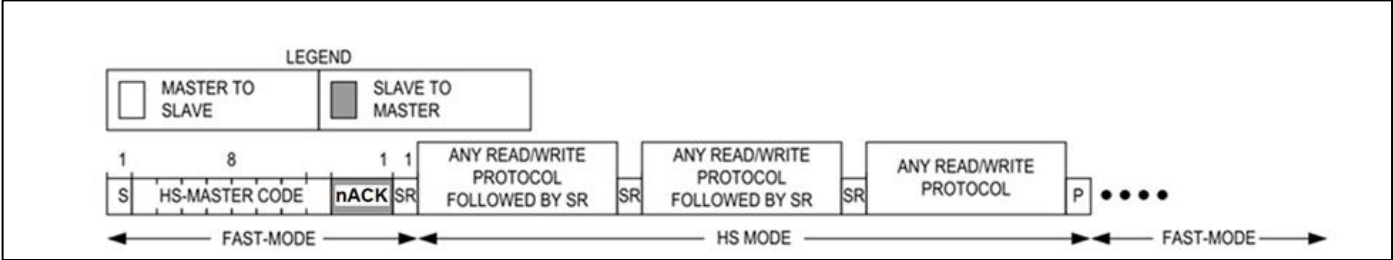
Figure 11. Engaging HS Mode
