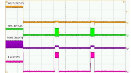
Time-5ms/div
