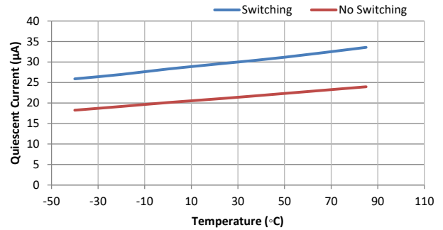
Supply Current (Quiescent), PFM
