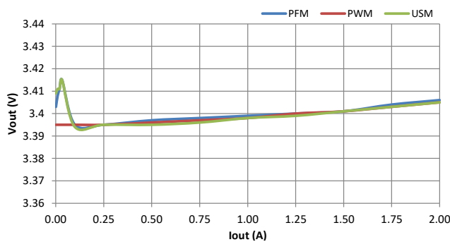
Load Regulation, P VIN =2.7V, V OUT =3.4V
