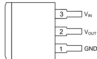
TO-263-3 (SA Package)
