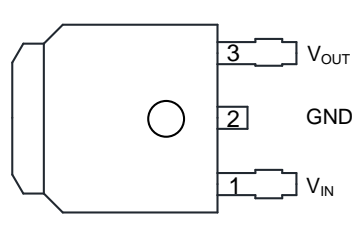
TO-252-2 (4)
