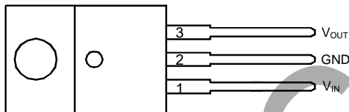
TO-220-3
