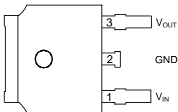
TO-252-2 (3)
