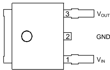
TO-252-2 (2)
