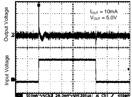
Line Transient
