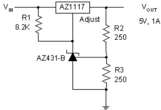
Precision 5V 1A Regulator
