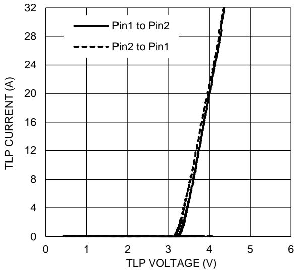
Figure 5 TLP Curve ( t_p = 100ns )
