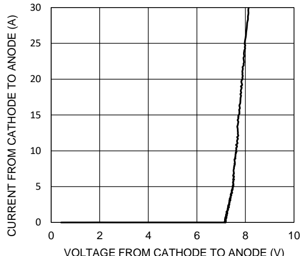
Figure 6 Current vs. Voltage (TLP, tp = 100ns)
