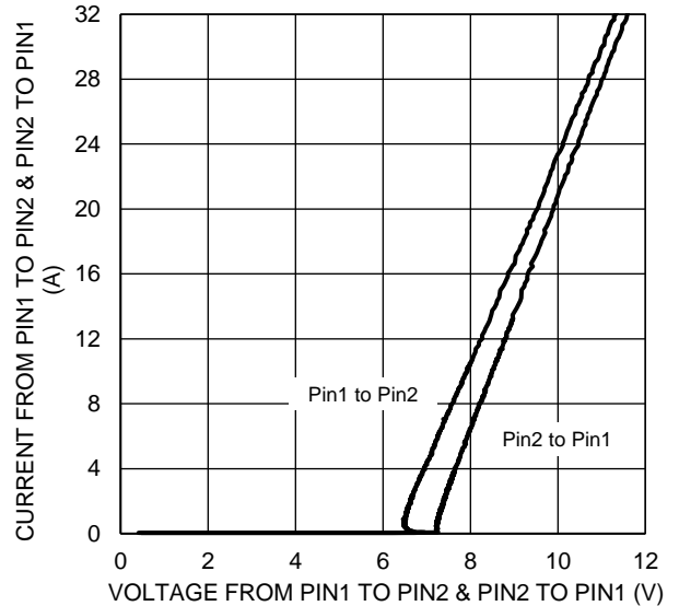
Figure 4 TLP Curve (t p = 100ns)
