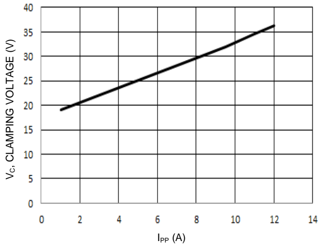
Figure 7. Clamping Voltage Characteristics ( t_p = 8/20\mu s )
