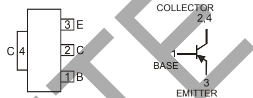
Schematic and Pin Configuration
