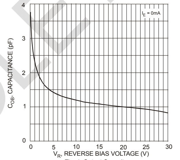
Fig. 4 Output Capacitance
