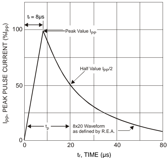
Figure 1. Pulse Waveform
