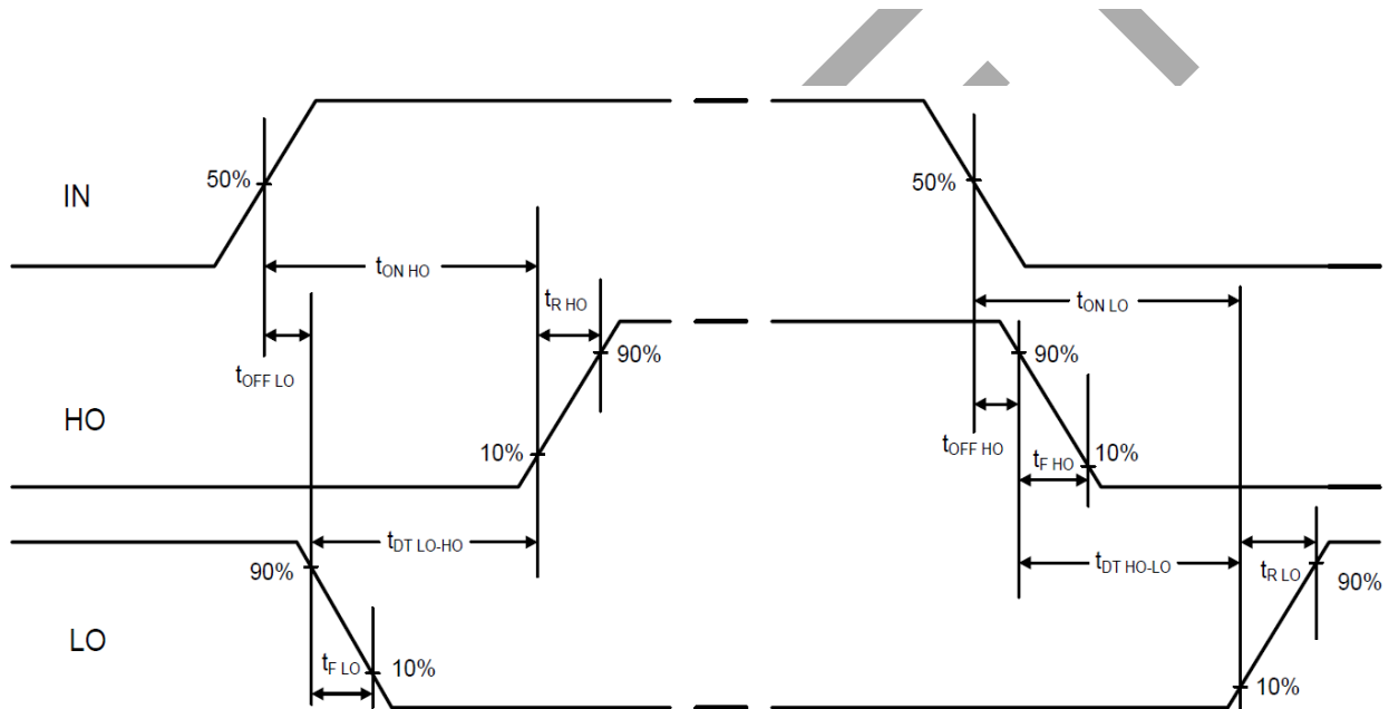
Figure 1. Input / Output Timing Diagram
