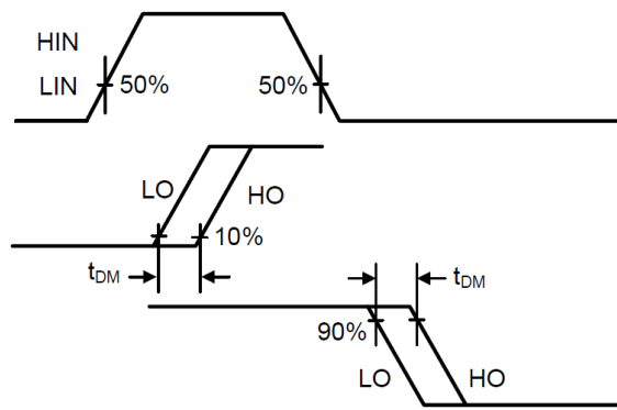
Figure 3. Delay Matching Waveform Definitions
