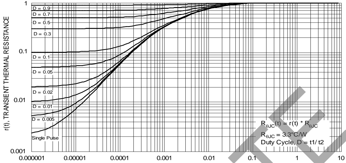
Figure 13 Transient Thermal Resistance
