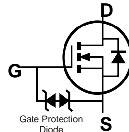
Equivalent Circuit
