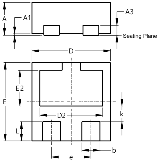
X2-DFN1010-3
