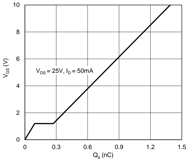
Figure 11. Gate Charge
