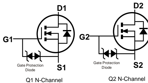
Equivalent Circuit
