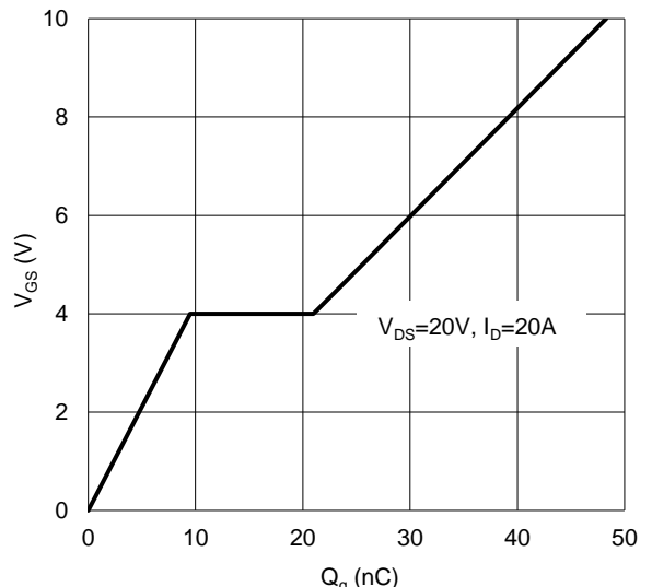
Figure 12. Gate Charge
