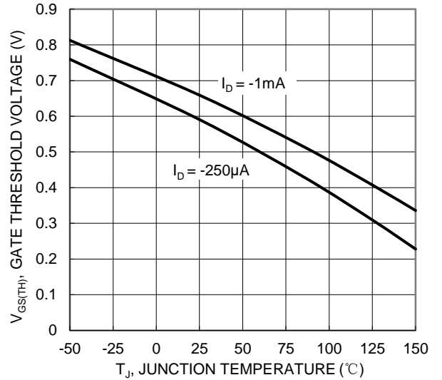
Figure 8. Gate Threshold Voltage vs. Junction Temperature
