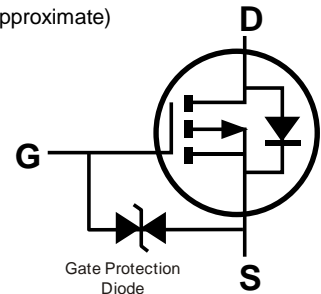
Equivalent Circuit
