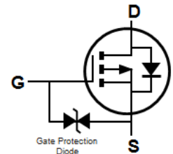
Equivalent Circuit
