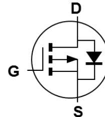
Equivalent Circuit
