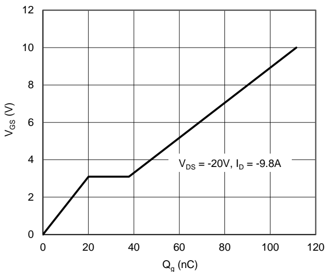
Figure 11. Gate Charge
