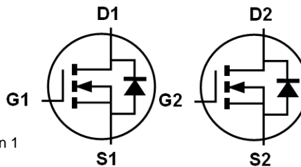
Equivalent Circuit
