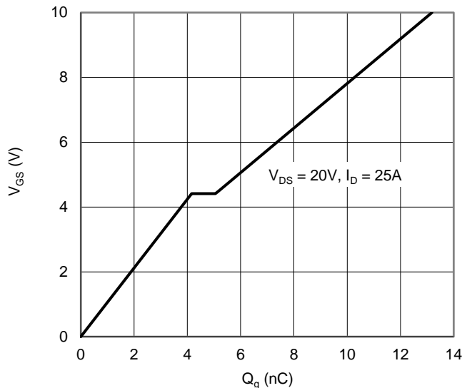
Figure 11. Gate Charge
