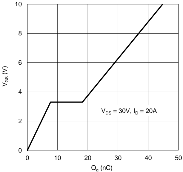
Figure 11. Gate Charge
