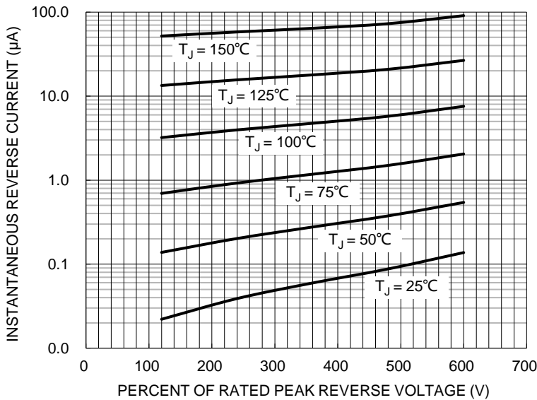
Figure 5. Typical Reverse Characteristics
