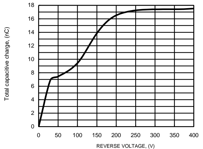
FIG.6 TYPICAL CAPACITIVE CHARGES
