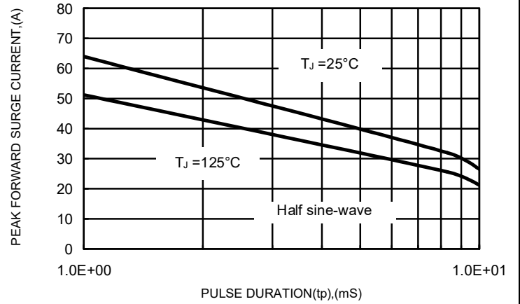
FIG.2 NON-REPETITIVE SURGE FORWARD CURRENT
