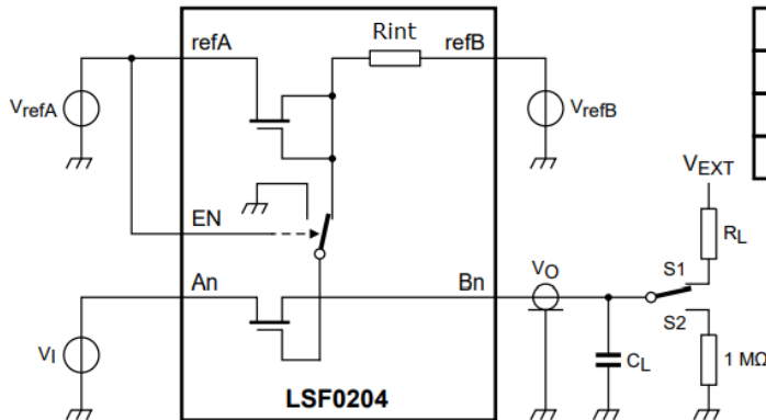
Test circuit
